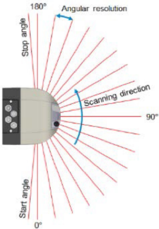
Figure: Angular resolution
