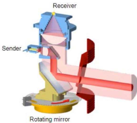
Figure: 2D laser scanner principle
