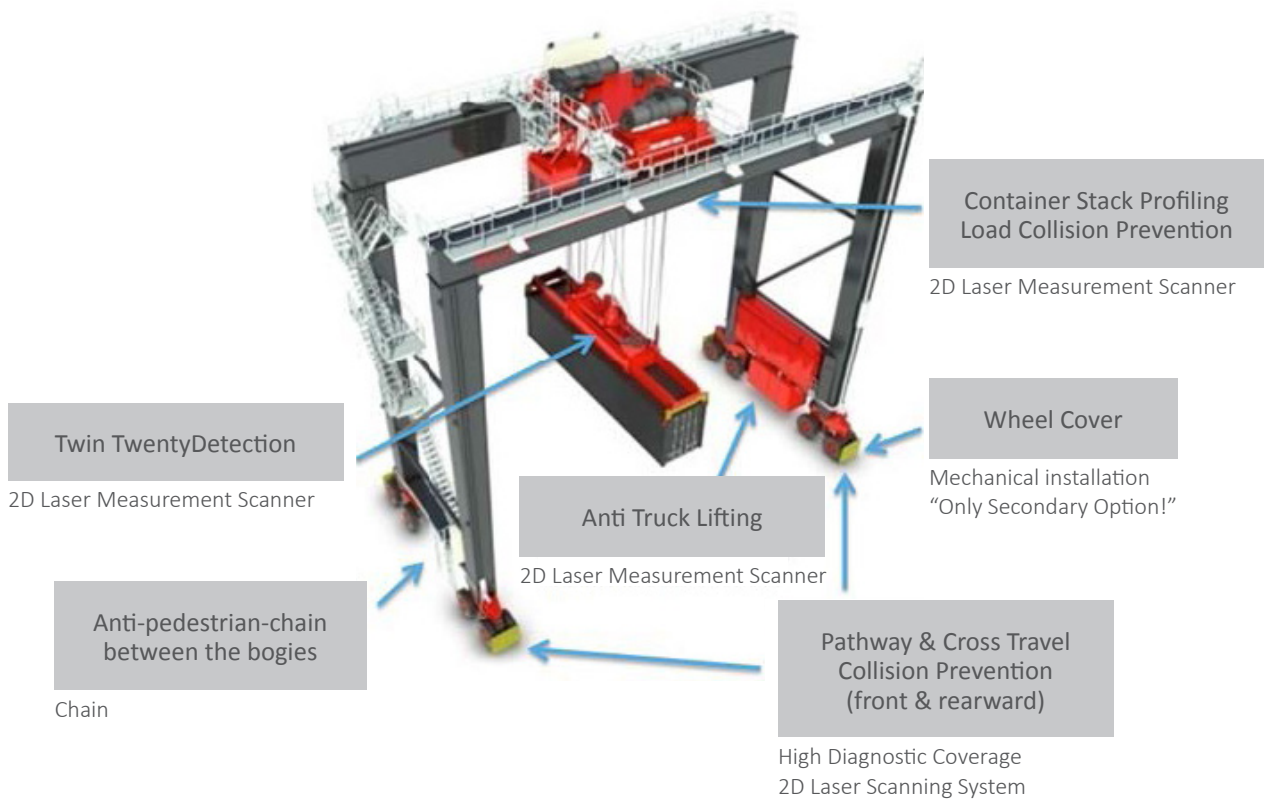
Figure: Collision Prevention Solutions at RTG
