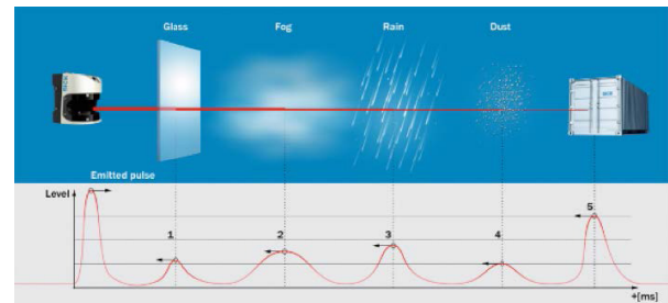
Figure: Multi-echo technology
