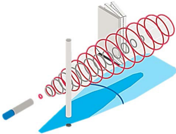
(Sonic) time-of-flight measurement
