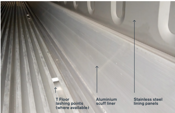
Picture 3 Interior floor/sidewall interface showing lashing points and exposed metal surfaces. Note that there may be no lashing points in the floor.
